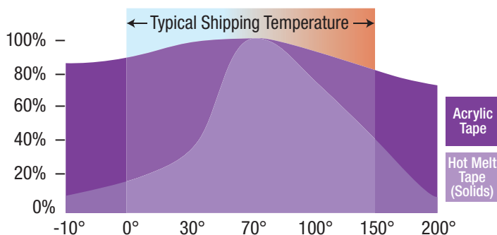
Box Closing Power (Cohesive Strength) of Tapes at Extreme Temperatures*
